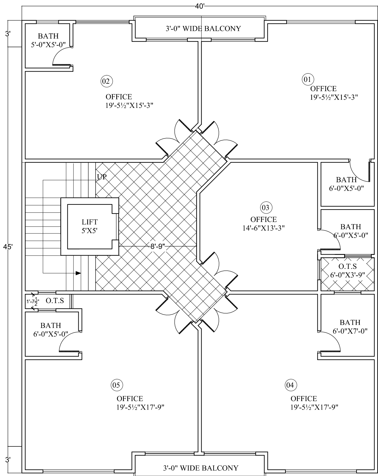
MEZZANINE FLOOR PLAN
